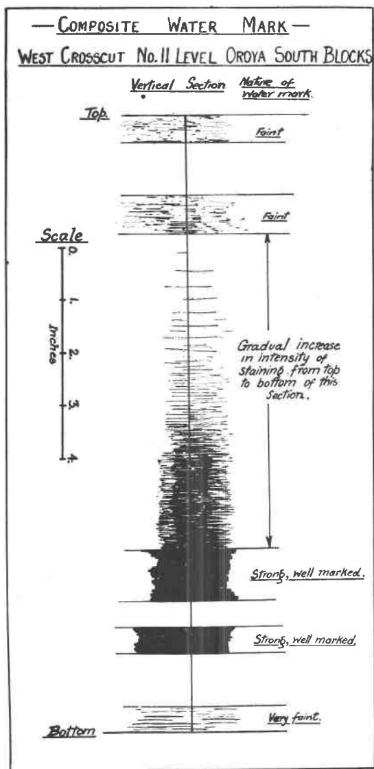
FIG. 5. Detailed section of the composite water line showing the distinguishable water marks due to changes in pressure in the airlock, No. 11 level, Oroya South Blocks mine. (From data supplied by Mr. A. Blatchford.)
