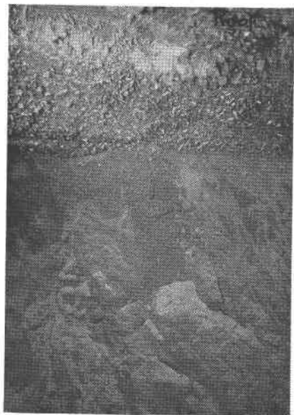
A. Photograph of wall of west crosscut, No. 11 level, Oroya South Blocks Mine, showing the profuse growth of gypsum crystals above the water line and their absence below.
